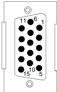
Figure B-1 Pin Layout and Pin Assignment Chart
